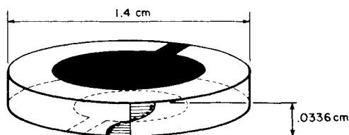
Fig. 5 Quartz crystal.
