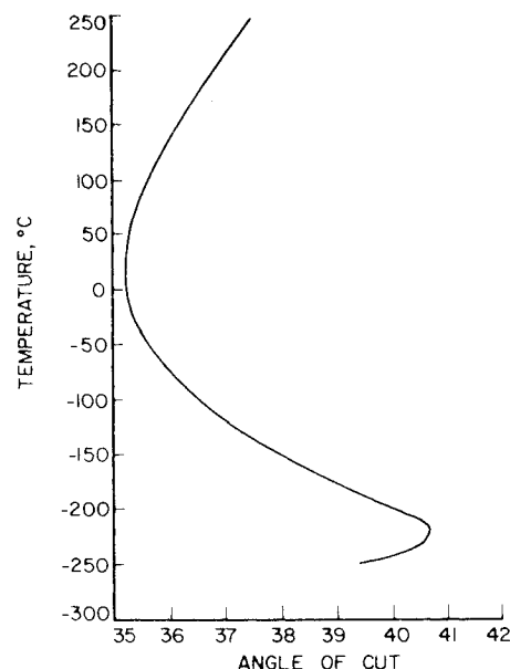
Fig. 3 Temperature for zero temperature coefficient.
