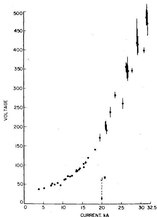
Fig. 7 Voltage-current characteristics; \dot{m} = 5 g/s.
